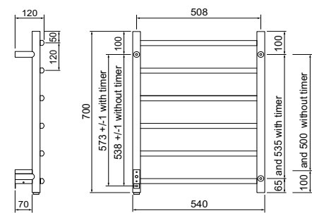
View from behind. Stated dimensions may vary. Never drill holes in the wall without first checking the dimensions of your actual towel warmer.
