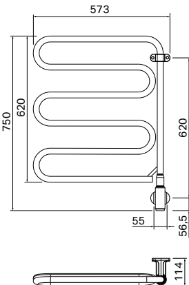
Stated dimensions may vary. Never drill holes in the wall without first checking the dimensions of your actual towel warmer.
