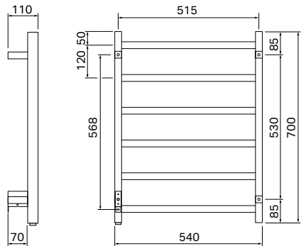
View from behind. Stated dimensions may vary. Never drill holes in the wall without first checking the dimensions of your actual towel warmer.
