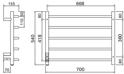
View from behind. Stated dimensions may vary. Never drill holes in the wall without first checking the dimensions of your actual towel warmer.
