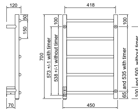
View from behind. Stated dimensions may vary. Never drill holes in the wall without first checking the dimensions of your actual towel warmer.
